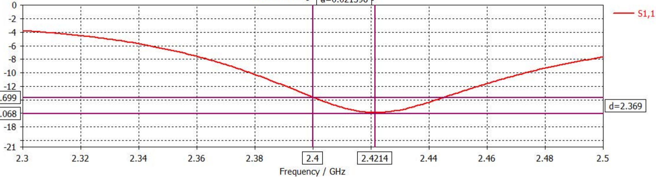
S-Parameters [Magnitude in dB]
