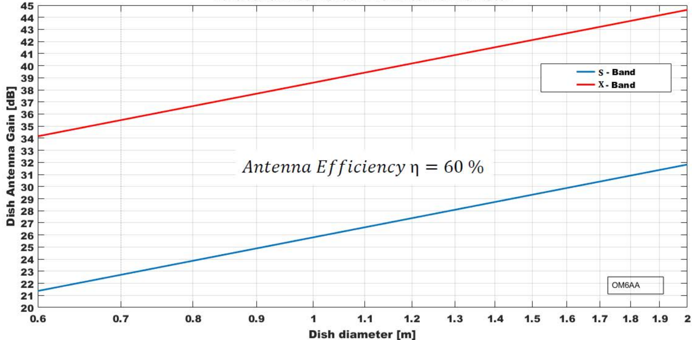
Parabolic Antenna Gain vs Antenna Diameter
