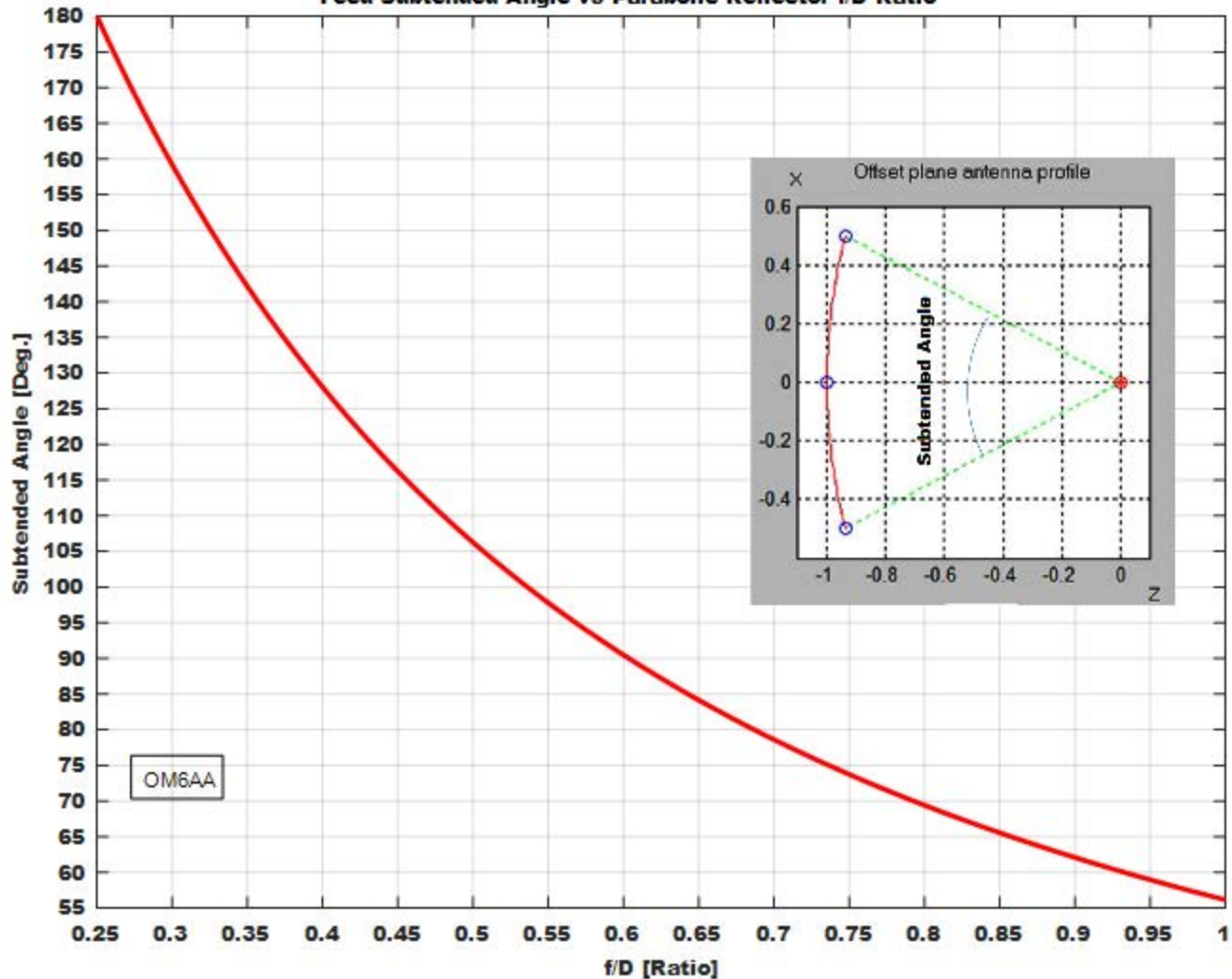
Feed Subtended Angle vs Parabolic Reflector f/D Ratio
