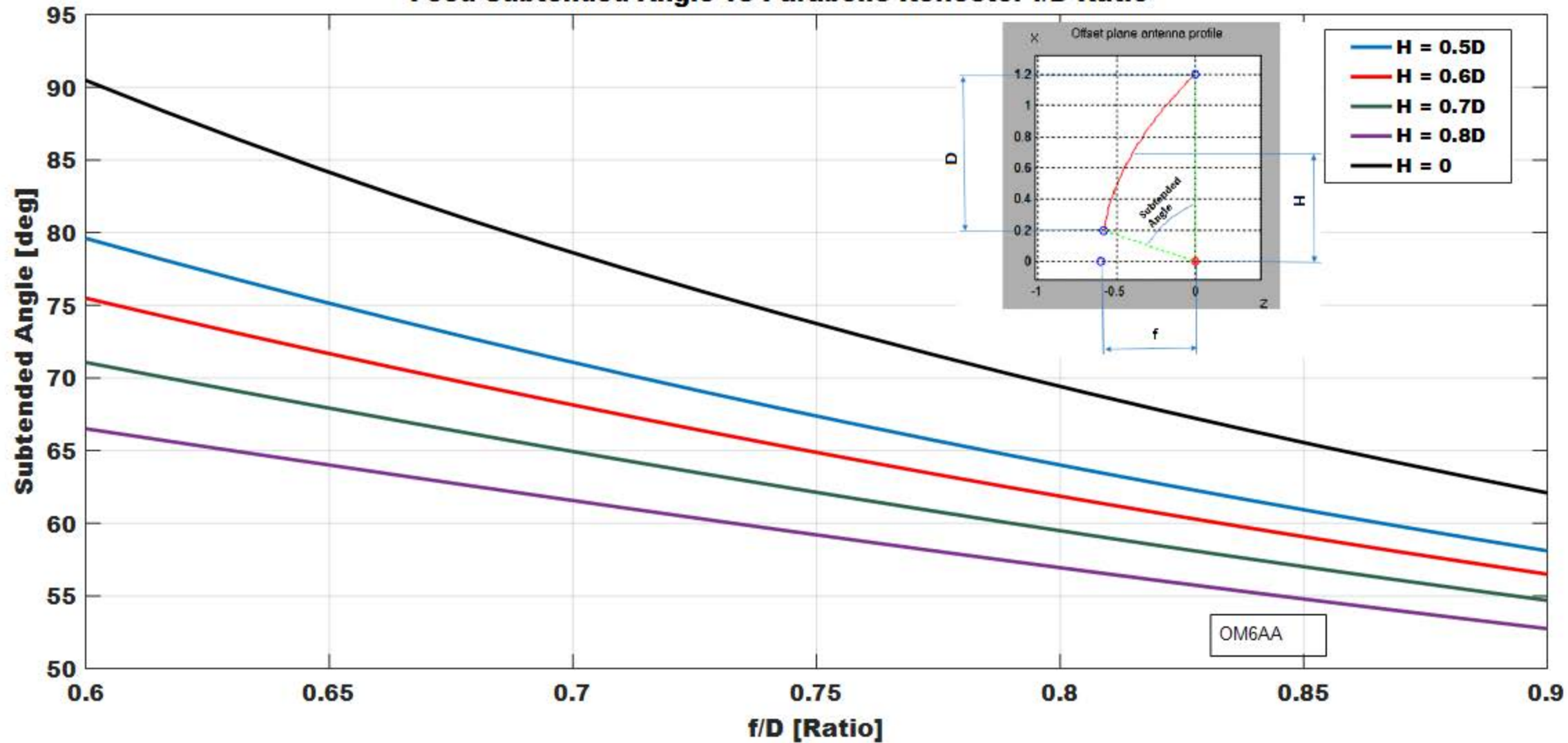
Feed Subtended Angle vs Parabolic Reflector f/D Ratio
