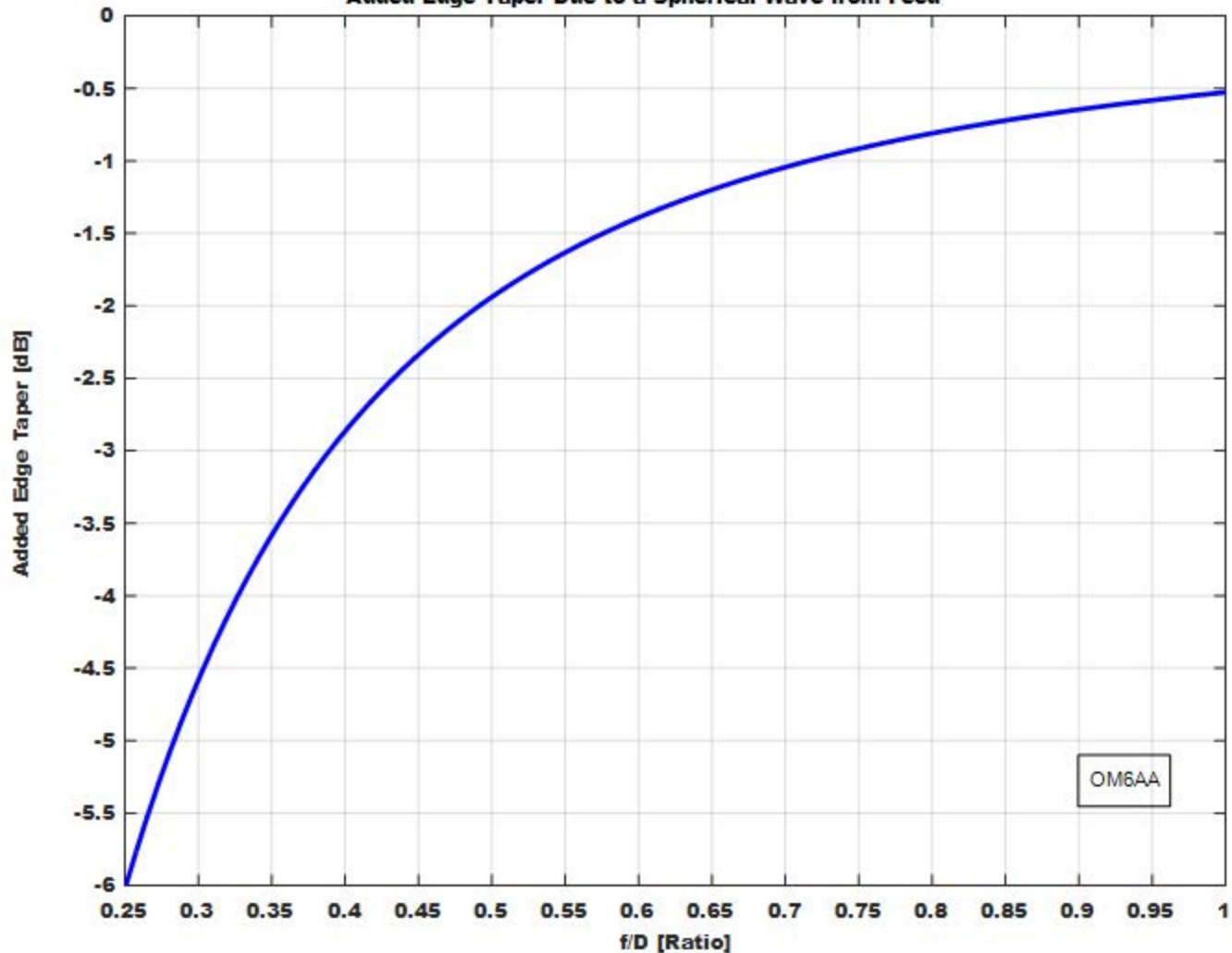
Added Edge Taper Due to a Spherical Wave from Feed
