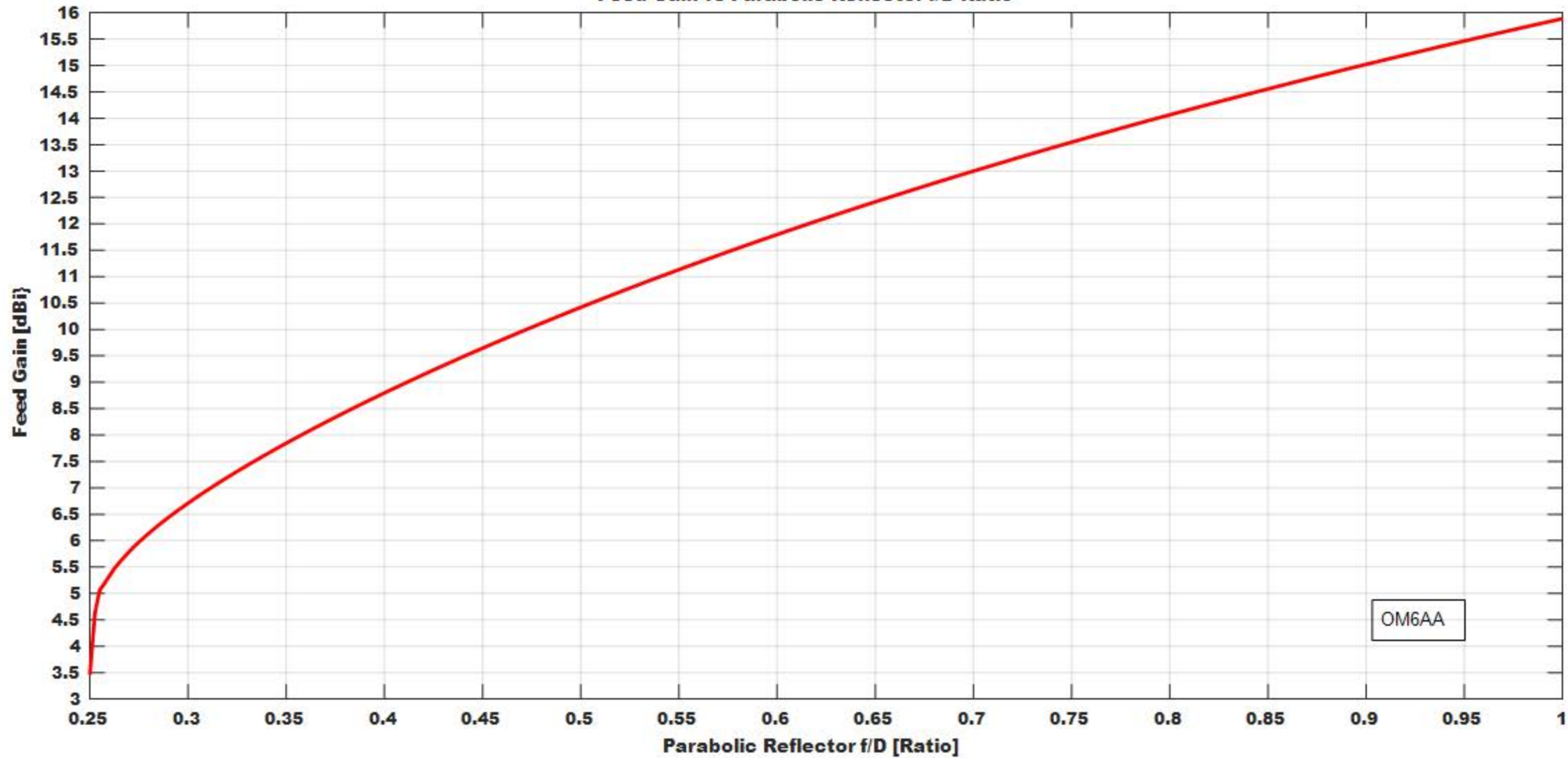
Feed Gain vs Parabolic Reflector f/D Ratio
