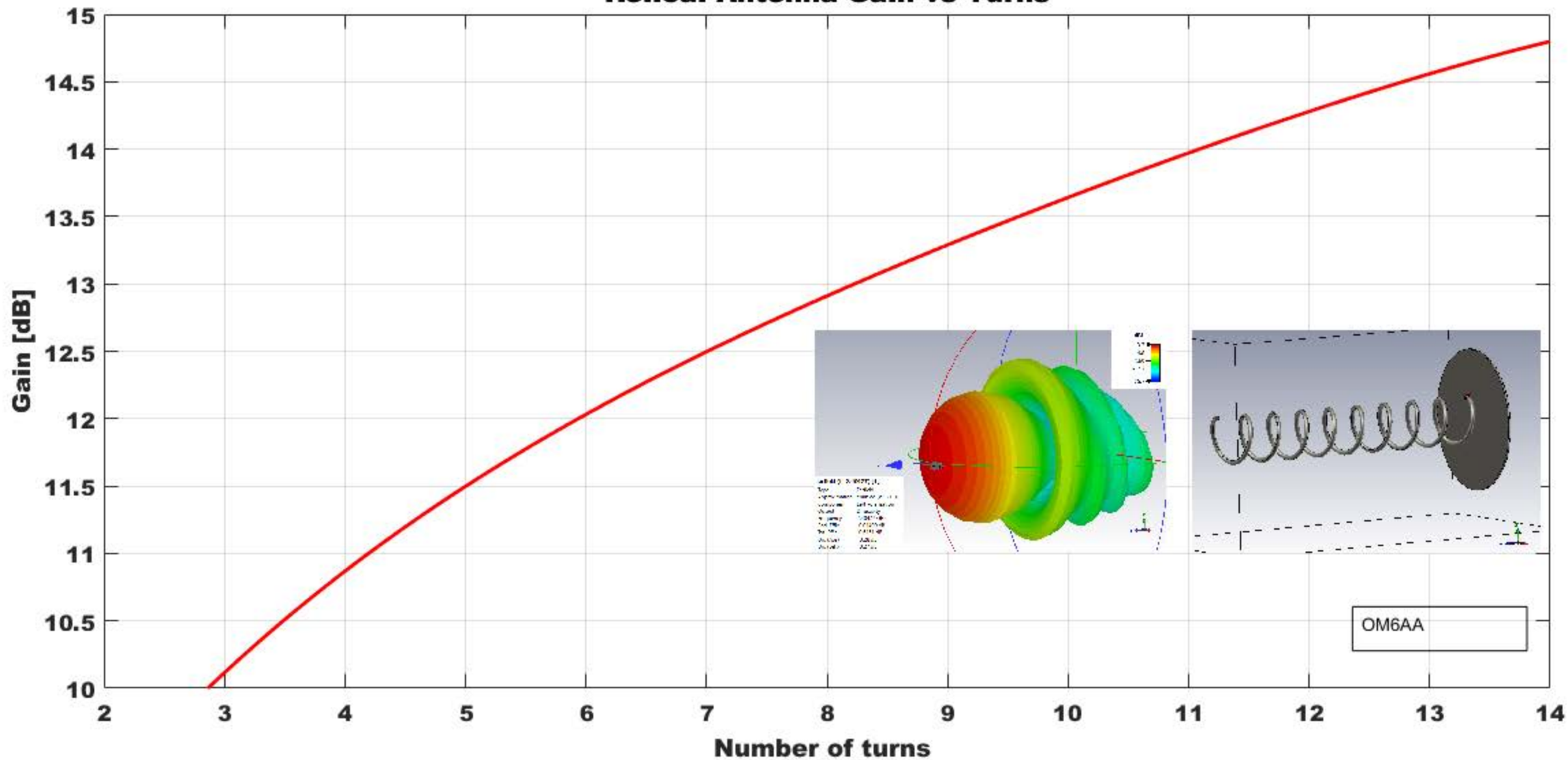
Helical Antenna Gain vs Turns
